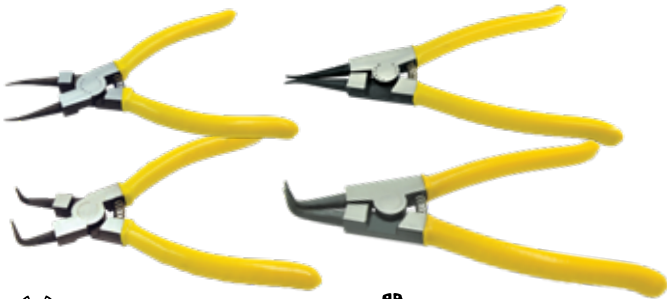
To assemble internal circlips into bore
